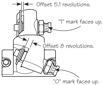
Figure 10: Blade offsets for 3/4" dowel.
