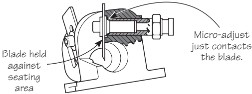
Figure 8: Zeroing the blades.
