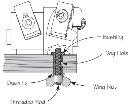
Figure 3: Dowel maker mounted with dog-hole mount assembly.
