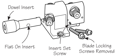
Figure 18: Removing blade assemblies.
