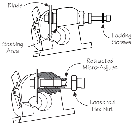
Figure 7: Resetting the micro-adjust.
