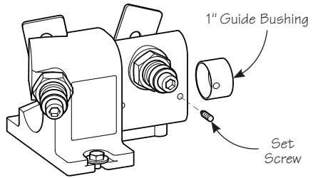
Figure 16: Guide bushing installation.
