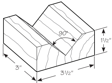
Figure 5: Shop-made dowel support.
