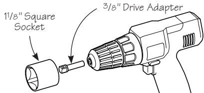
Figure 13: Drive adapter and square socket.
