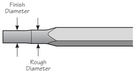
Figure 15: Rough and final diameters.
