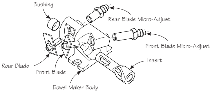
Figure 1: Exploded view of Veritas® Dowel Maker.
