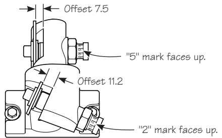
Figure 12: Blade offsets for 1" dowel.
