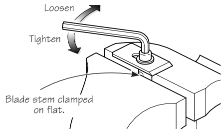
Figure 20: Removing the blade from its mounting stem.
