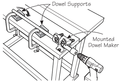
Figure 4: Typical set-up for running dowel.
