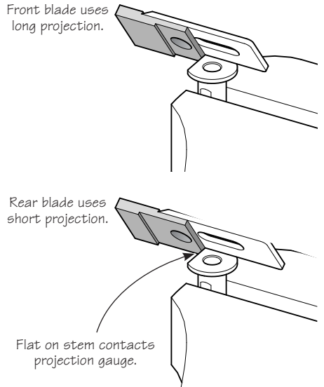
Figure 21: Blade-setting gauge on front blade.
