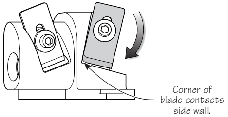
Figure 11: Positioning the front blade.
