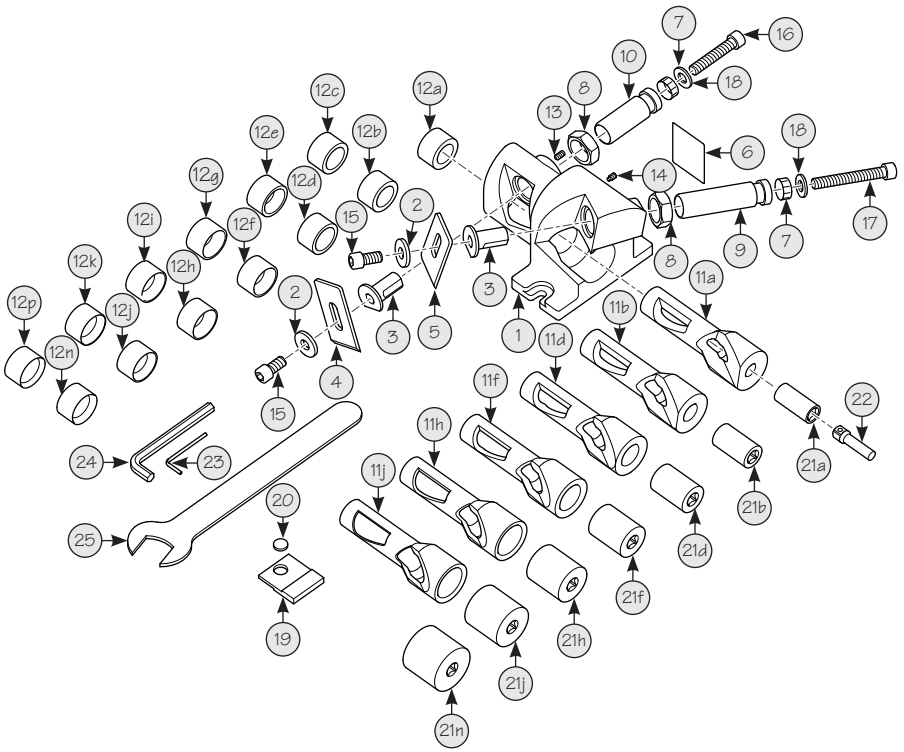
Figure 22: Exploded parts diagram.
