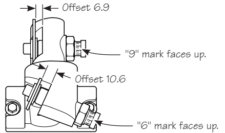
Figure 17: Blade offsets for 15/16" dowel.
