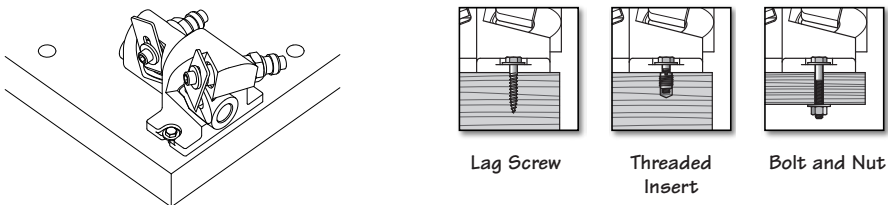
Figure 2: Dowel maker mounting options.
