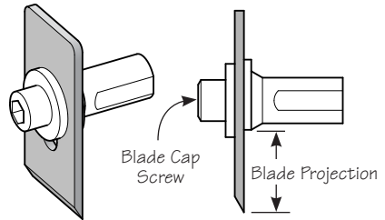
Figure 6: Blade cap screw and projection.
